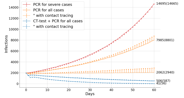
Fig. 7. As in Fig. 1, change to dots and numbers in parentheses show only one screening test for mild and moderate cases.
