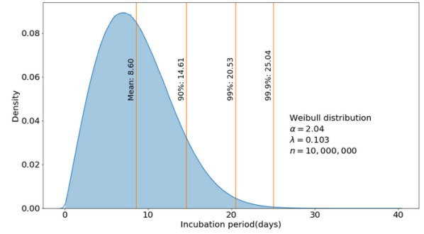
Fig. 5. The incubation period used in the model [13]
