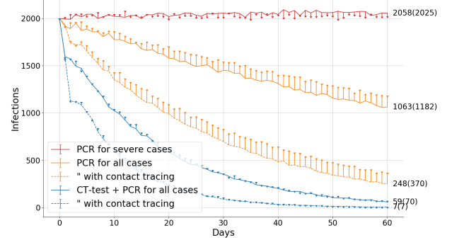
Fig. 8. As in Fig. 2, change to dots and numbers in parentheses show only one screening test for mild and moderate cases.
